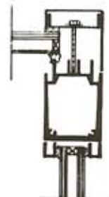
CROSS BAR - DETAILS 3
