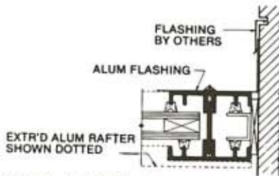
HEAD - DETAILS 6
