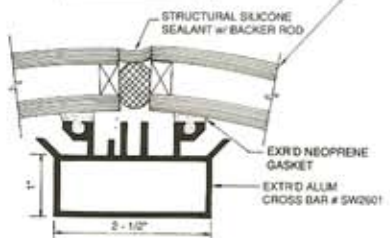
CROSS BAR - DETAILS
