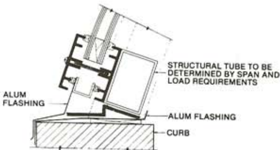
CURB - DETAILS 4
