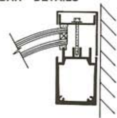
HEAD - DETAILS 6
