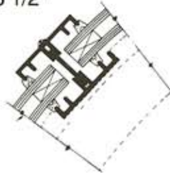
CROSS BAR - DETAILS 3
