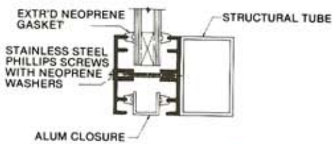
END CURB - DETAILS 2
