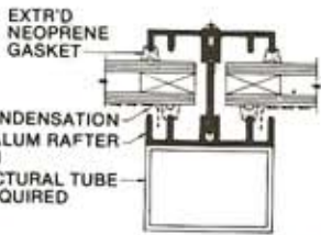
MAIN RAFTER - DETAILS 5
