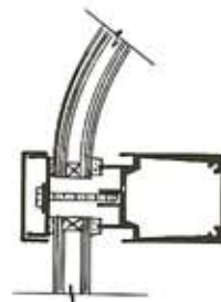
CROSS BAR - DETAILS 3
