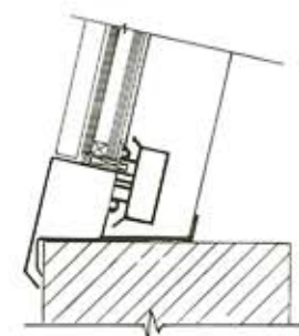
SEGMENTED VAULT SILL - DETAIL 3
